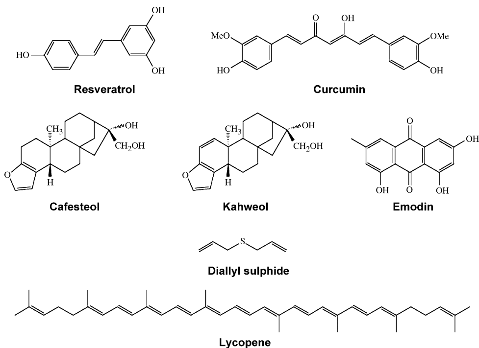
Fig. 2. Molecular structure of selected chemopreventive agents.
