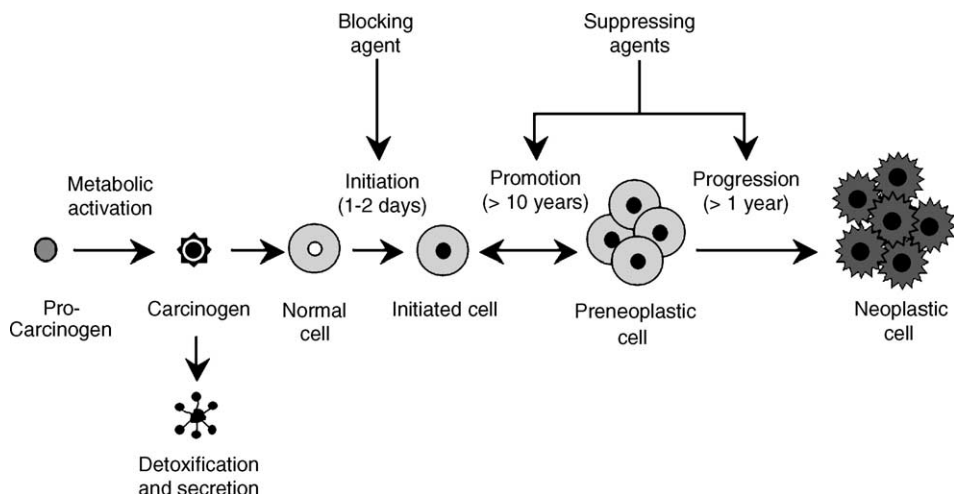
Fig. 1. Schematic representation of multistep-carcinogenesis (from Surh et al. with modifications [69]).
